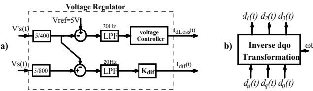
Fig. 7 – (a) Voltage regulator; (b) Inverse dq0 transformation.
