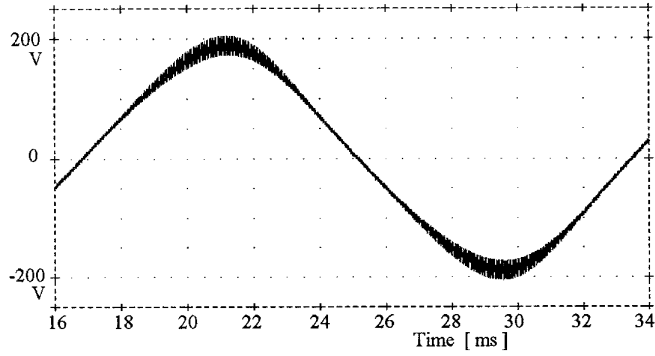
Fig 11. Output voltage.
