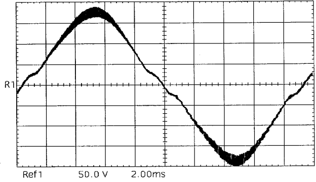
Fig 15 Output voltage
