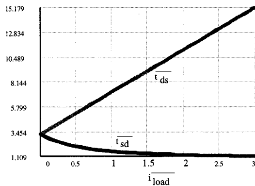
Fig. 5. Total commutation durations for diode to switch commutation ( t_{ds} : t_6-t_1 ) and switch to diode commutation ( t_{sd} : t_{10}-t_7 ) versus load current.
