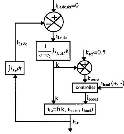
Fig. 12. DC center potential control system including the intrinsic neutral line current feedback loop and the extrinsic dc center potential voltage feedback loop.
