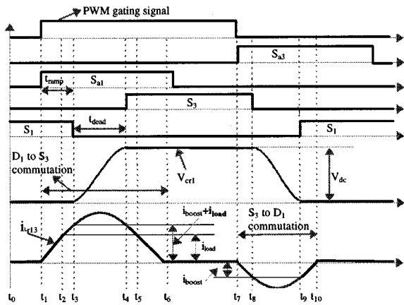
Fig. 2. Predicted waveforms for commutations between S_1/D_1 and S_3/D_3 when the load current is negative ( D_1 \leftrightarrow S_3 ). Note that “ i_{boost} ” for switch to diode commutation is equal to the “ i_{boost} ” for diode to switch commutation, and is consistently applied without regard to the level of the load current.
