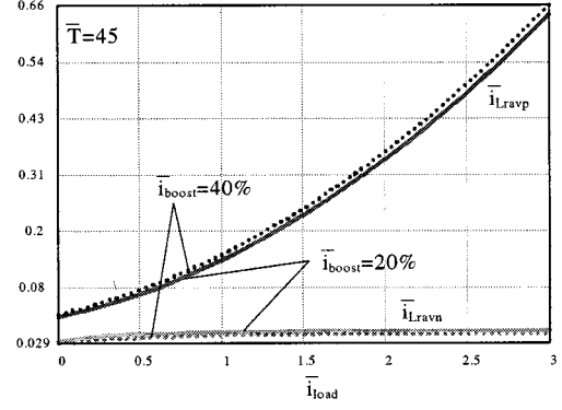
Fig. 11. Resonant inductor average current averaged over the switching cycle versus load current, switching cycle, and \bar{i}_{boost} for diode to switch commutation ( \bar{i}_{Lravp} ) and switch to diode commutation ( \bar{i}_{Lravm} ).
