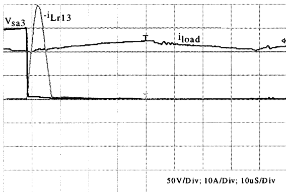
Fig. 14. Experimental voltage and current waveforms of the auxiliary switch S_{a3} during D_{c1} to S_1 commutation in relation to the load current. Auxiliary switches work with inductive turn-on and zero-current turn-off. Besides, the auxiliary switches block only half of the main switches blocking voltage.
