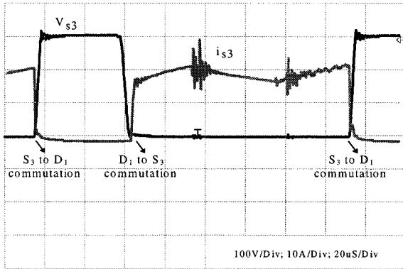
Fig. 13. Experimental voltage and current waveforms of the inner main switch S_3 during D_1 to S_3 and S_3 to D_1 commutations. Main switches work with capacitive turn-off and zero-voltage turn-on. Besides, static overvoltage problem of the inner switches has been resolved by the clamping resistor R_c .
