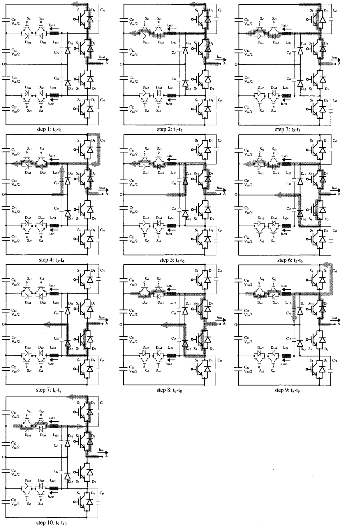
Fig. 3. Step diagram for commutations between D_1 and S_3 in the proposed ARCPNPC inverter when the load current is negative.
