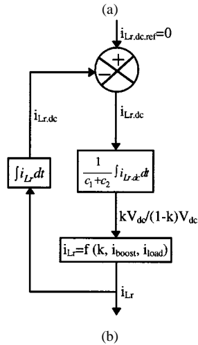
Fig. 10. (a) Resonant inductor average current \bar{i}_{Lrav} solved over the switching cycle flowing out of the dc center potential corresponding to positive load current versus load current and dc-link voltage distribution factor k . (b) Neutral line current feedback loop and self-balancing of the dc center potential in the basic ARCPI circuit.
