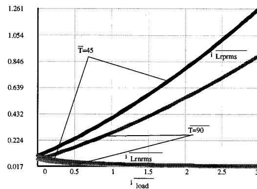
Fig. 7. Resonant inductor rms currents solved over the switching cycle for diode to switch commutation ( \overline{i_{Lrprms}} ) and switch to diode commutation ( \overline{i_{Lrnms}} ) versus load current and switching cycle.
