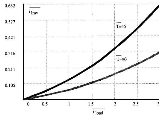
Fig. 8. Resonant inductor average current \overline{i_{Lrav}} solved over the switching cycle flowing out of the center potential corresponding to positive load current versus load current and switching cycle.
