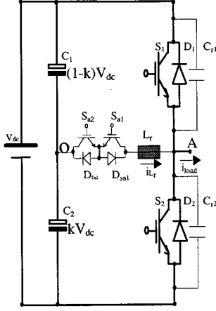
Fig. 9. Basic ARCPI circuit structure with dc voltage distribution factor of k .
