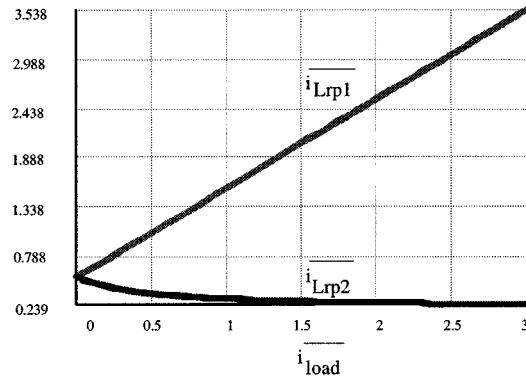
Fig. 6. Resonant inductor peak currents solved over the switching cycle for diode to switch commutation ( \overline{i_{Lrp1}} ) and switch to diode commutation ( \overline{i_{Lrp2}} ) versus load current.
