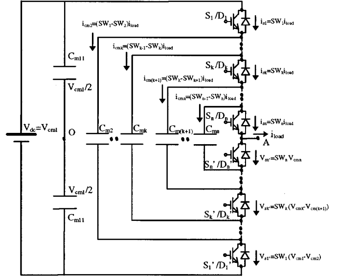
Fig. 4. Configuration of a half-bridge (n + 1) -level capacitor-clamping-inverter.
