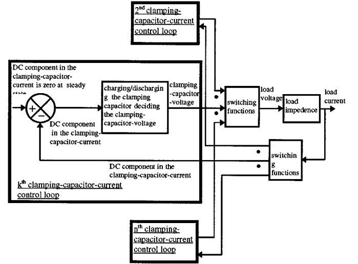
Fig. 5. Coupled spontaneous clamping-capacitor-current control loops in the half-bridge (n + 1) -level capacitor-clamping-inverter.
