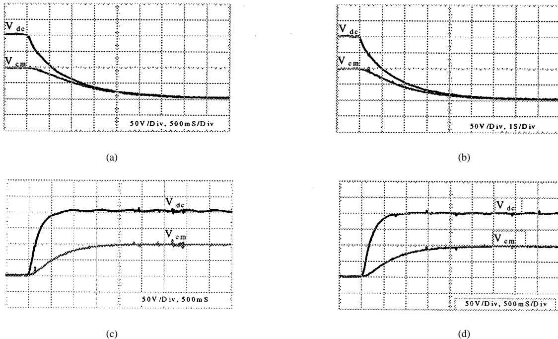
Fig. 6. Test results of the clamping-capacitor-voltage self-balancing in the half-bridge capacitor-clamping-inverter, with different load resistances when the dc supply is switched off and on: (a) dc supply switched off, load resistance R_o = 3 \Omega , (b) dc supply switched off, load resistance R_o = 7.5 \Omega , (c) dc supply switched on, load resistance R_o = 3 \Omega , and (d) dc supply switched on, load resistance R_o = 7.5 \Omega .
