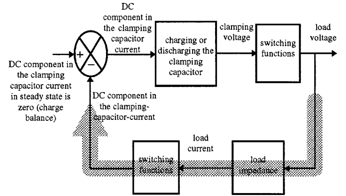
Fig. 3. Spontaneous clamping-capacitor-current control loop in the half-bridge three-level capacitor-clamping-inverter.
