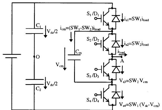
Fig. 1. Structure of a half-bridge three-level capacitor-clamping-inverter.
