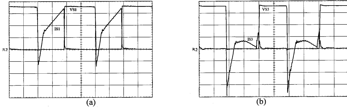
Fig. 7. Voltage and current waveforms in full-load condition: (a) main switch S_1 (scales: 100 V/div., 10 A/div., 10 us/div.), (b) auxiliary switch S_3 (scales: 100 V/div., 10 A/div., 10 us/div.).
