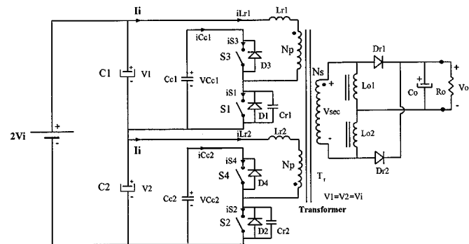
Fig. 1. Proposed dc–dc converter.
