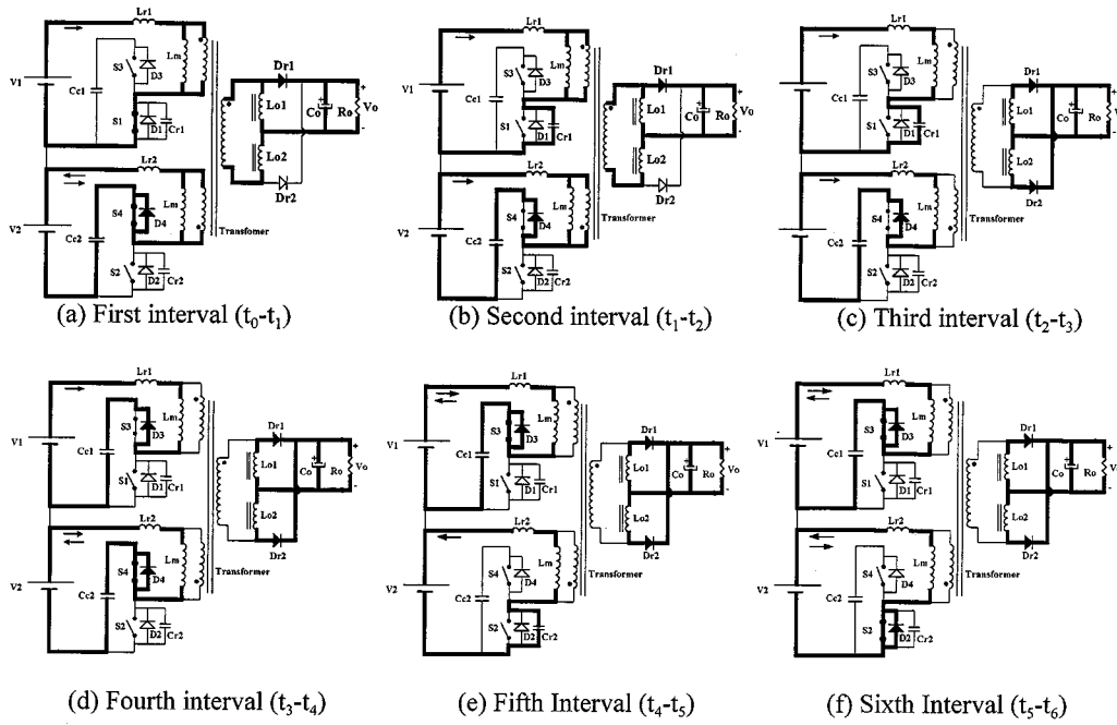
Fig. 2. Topological operation states of the proposed converter.
