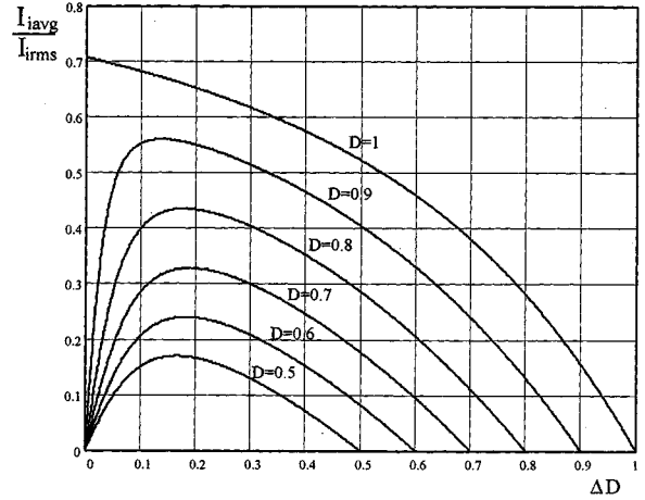
Fig. 6. Average and rms input current ratio.
