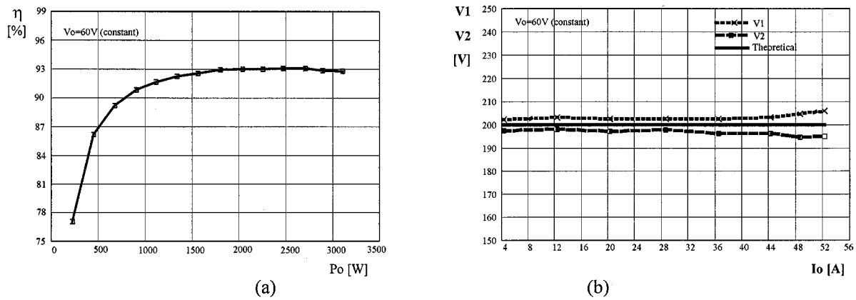
Fig. 11. Experimental curves of (a) measured efficiency of the converter and (b) voltages across input capacitors C_1 and C_2 .
