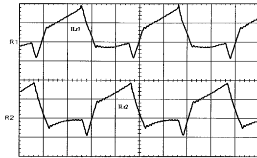
Fig. 9. Currents through inductors L_{r1} and L_{r2} in full-load condition (scales: 20 A/div., 10 us/div.).
