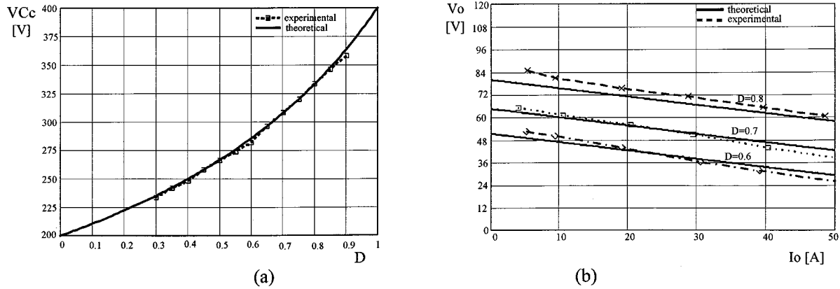
Fig. 10. Experimental curves of (a) clamping characteristic and (b) output characteristic.
