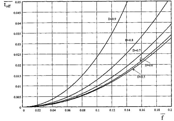
Fig. 5. Normalized charge time interval \bar{t}_{off} , as a function of \bar{f} , during turn-off.
