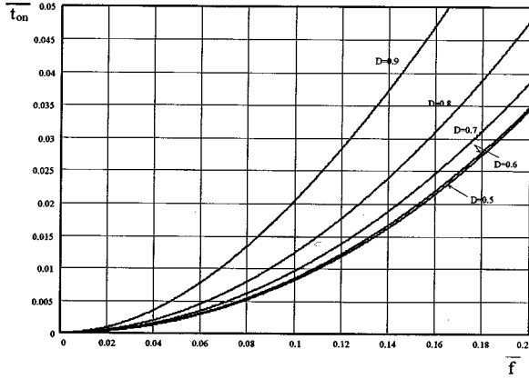
Fig. 4. Normalized discharge time interval \bar{t}_{on} , as a function of \bar{f} , during turn-on.
