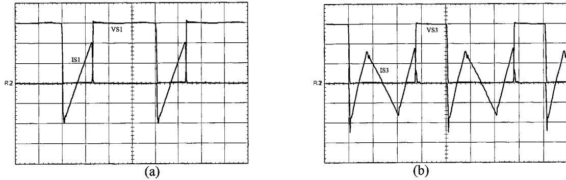
Fig. 8. Voltage and current waveforms in no-load condition: (a) main switch S_1 (scales: 100 V/div., 10 A/div., 10 us/div.), (b) auxiliary switch S_3 (scales: 100 V/div., 10 A/div., 10 us/div.).
