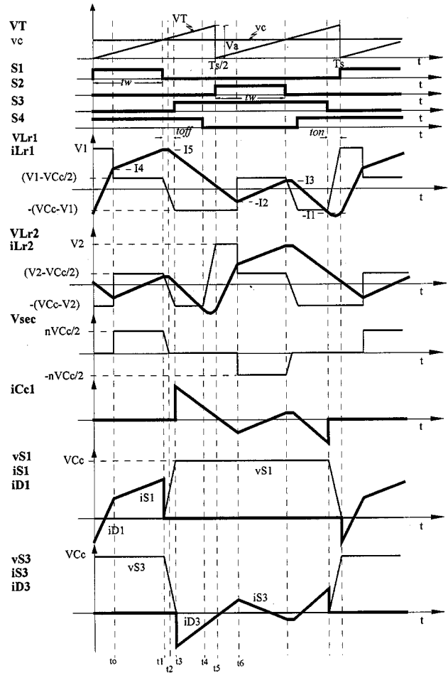
Fig. 3. Main waveforms of the proposed converter.
