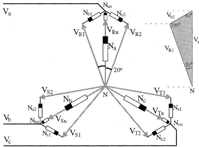
Fig. 3. Vector diagram and auxiliary triangle.
