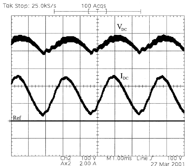
Fig. 10. DC-link voltage and current without series connection of the secondary windings. Scales: 1 ms/div, 100 V/div, 2 A/div.
