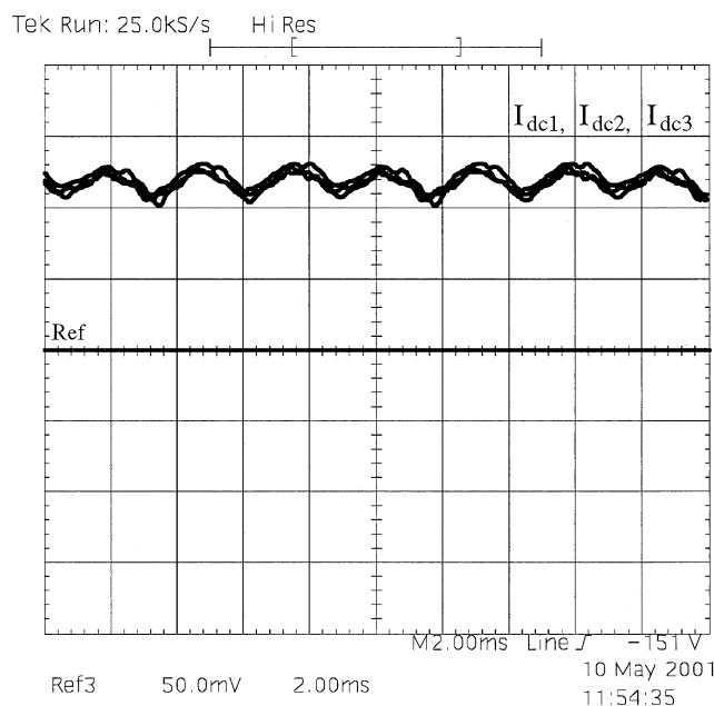
Fig. 11. Balanced dc-link currents. Scales: 2 ms/div, 5 A/div.
