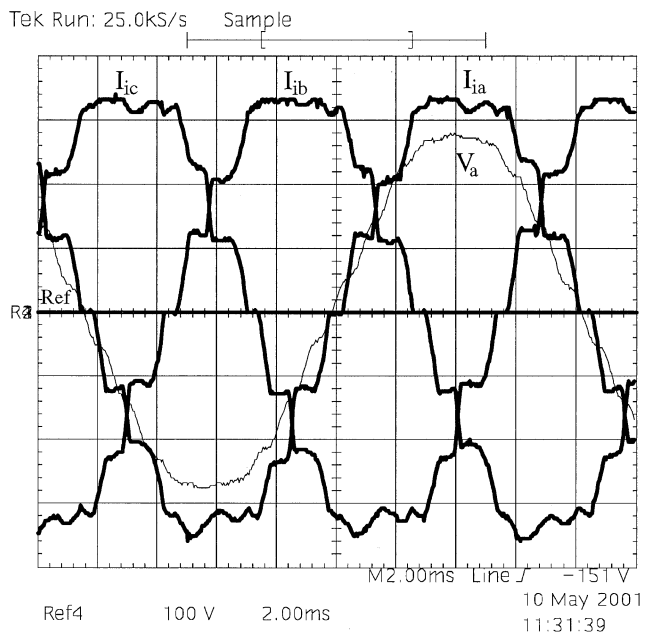
Fig. 15. Line currents. Scales: 2 ms/div, 10 A/div, 100 V/div.
