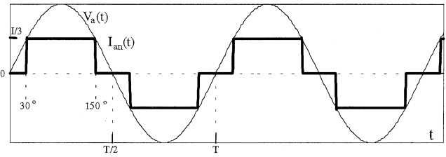
Fig. 4. Primary voltage and secondary current to phase "a."
