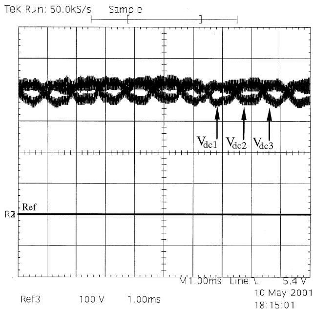
Fig. 13. Rectified voltages through dc-links. Scales: 1 ms/div, 100 V/div.
