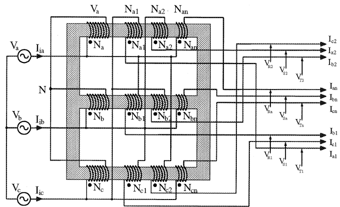
Fig. 2. Scheme of the autotransformer windings.
