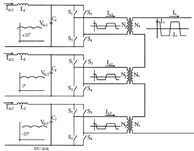
Fig. 8. Circuit to achieve balanced dc-link currents.
