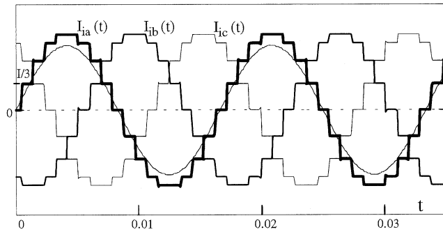
Fig. 6. Three-phase line currents and voltage of phase "a."
