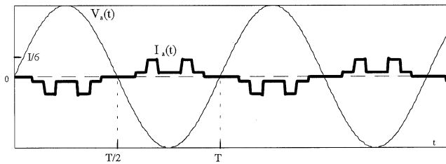
Fig. 5. Primary current to phase "a."
