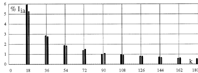
Fig. 7. Harmonics of line current I_{ia} .
