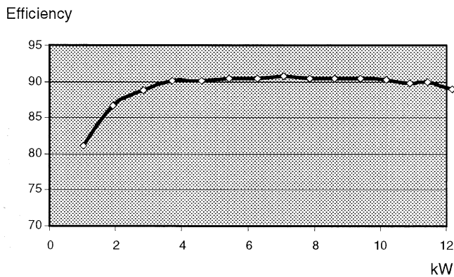
Fig. 16. Efficiency.
