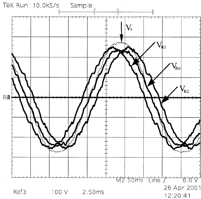
Fig. 12. Line voltage and input voltages of the diode rectifiers. Scales: 2.5 ms/div, 100 V/div.
