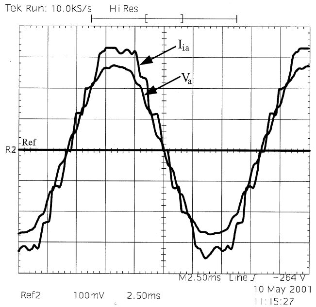
Fig. 14. Input current and input voltage in the same phase. Scales: 2 ms/div, 10 A/div, 100 V/div.
