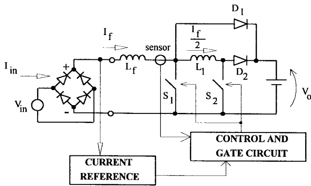
Fig. 17. A unity power factor rectifier based on a 2I boost converter.
