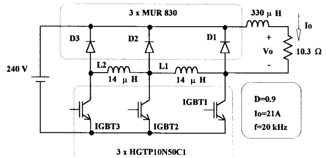
Fig. 13. 3I buck converter (experimental circuit).
