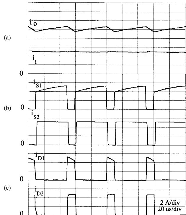
Fig. 9. Experimental selected waveforms for the 2I buck converter: (a) inductor currents, (b) IGBT collector currents, and (c) diode currents.
