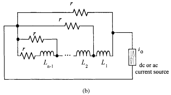
Fig. 3. Simplified equivalent circuit for: (a) 2I buck and (b) generic structure.
