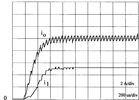
Fig. 10. Step-voltage response for the 2I-buck converter.
