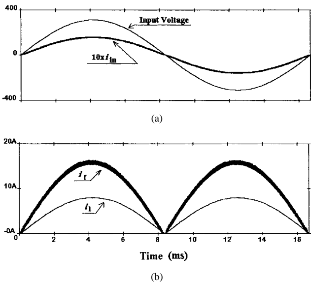
Fig. 18. Waveforms from computer simulation: (a) utility voltage and current and (b) boost and balance inductor currents.
