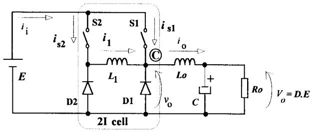
Fig. 2. DC-DC 2I buck converter.
