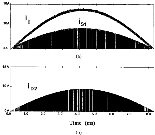
Fig. 19. Waveforms from computer simulation: (a) input inductor and S_1 currents and (b) D_2 current.
