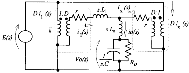
Fig. 5. Line-to-output model for 2I buck converter.
