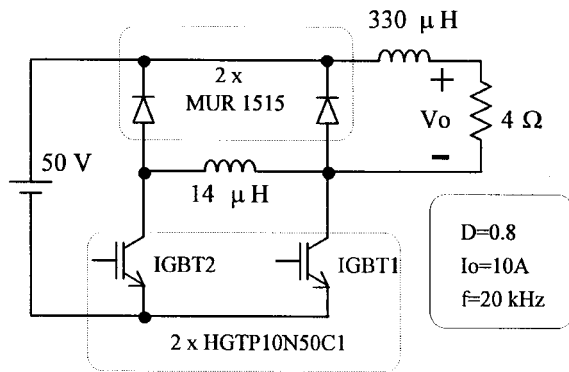
Fig. 8. Laboratory circuit.
