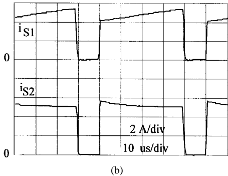
Fig. 12. Collector currents for nonsimultaneous gate pulses: (a) L_1 = 0 and (b) L_1 = 14 \mu\text{H} .
