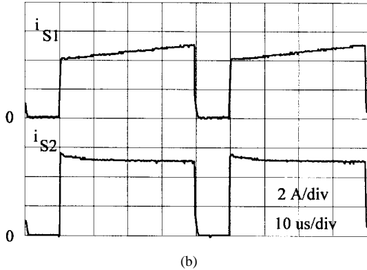
Fig. 11. Unbalanced emitter-ground experiment: (a) collector currents for L_1 = 0 and (b) collector currents for L_1 = 14 \mu\text{H} .
