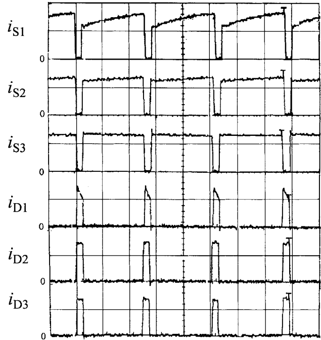
Fig. 14. Comparison among device currents (5 A/div, 20 \mu\text{s} /div).
