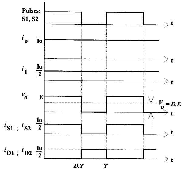
Fig. 4. Selected basic ideal waveforms.
