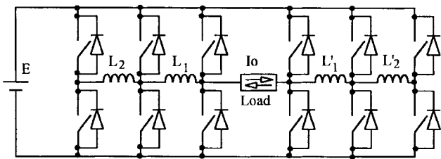
Fig. 16. Full-bridge 3I voltage source inverter.
